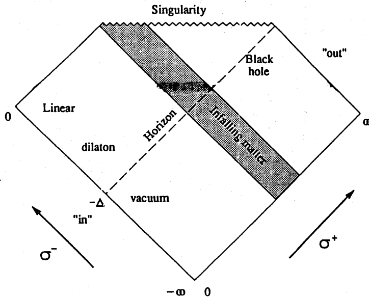
Fig. 5: The Penrose diagram for a collapsing black hole formed from a left-moving matter distribution.
