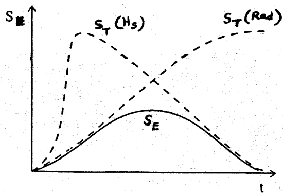
FIG. 8 Entanglement entropy of radiation and stretched horizon. The dashed curves indicate the thermal entropies
