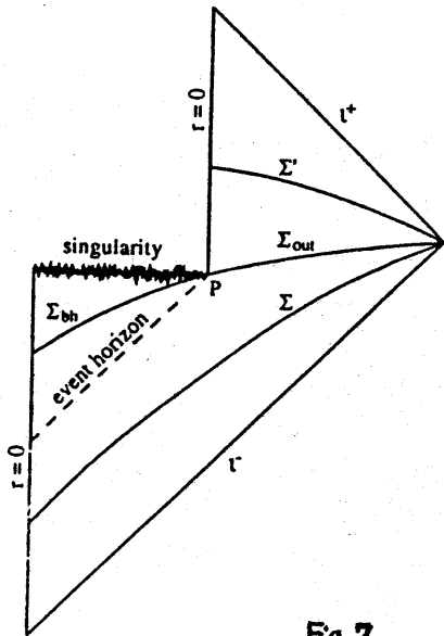
Penrose diagram for black hole evolution.
