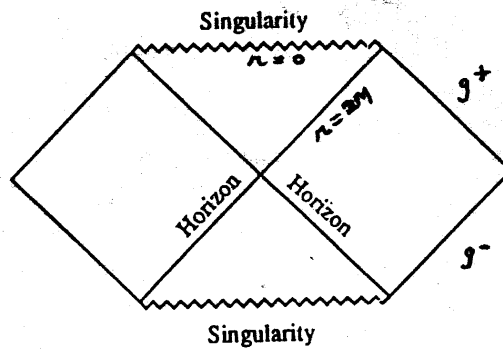
Fig. 2 Penrose diagram
