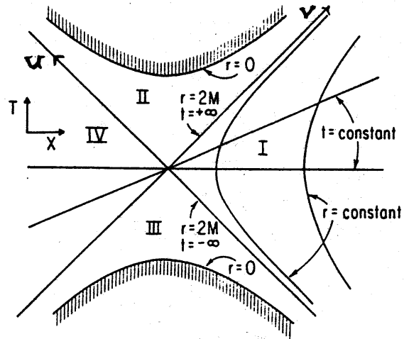
Fig. 1 The Kruskal extension of Schwarzschild spacetime.
